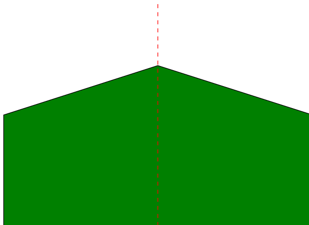
Figure 343: How the Midpoint Displacement Algorithm Works (2/4)
